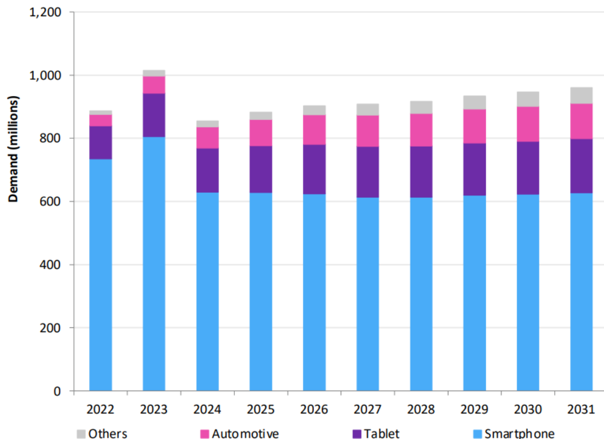
LCD TDDI demand forecast by application
